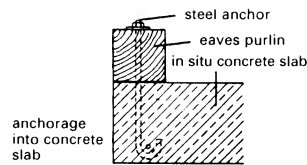
8 Anchorage to solid slab
